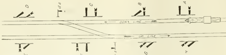
POSITION OF SIGNALS WITH "DOWN" CROSSOVER SWITCH OPEN.
